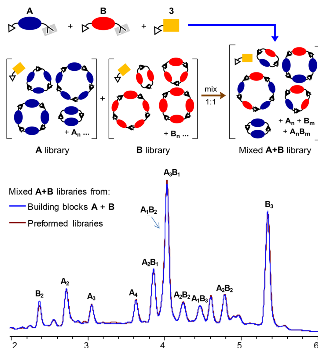
Figure 3. Applying equilibrators 3 afforded DCLs at thermodynamic equilibrium, as evidenced by the fact that mixed A + B libraries (1:1, 1.0 mM total building block concentration in CHCl 3 with 15 vol % methanol, 10 vol % acetonitrile, and 1 vol % TFA) reached the same composition whether they were started by combining the building blocks A and B or by mixing already formed libraries of A and B.
