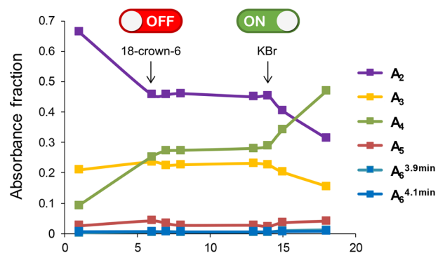
Figure 7. Composition of dynamic library of A (chromatograms at 325 nM) as a function of time (days). Addition of 18-crown-6 completely stops library evolution by effectively removing equilibrators 3 from the mixture. Library evolution is started again immediately upon addition of KBr to release 3 by competitive binding of 18-crown-6 by K^+ ions.
