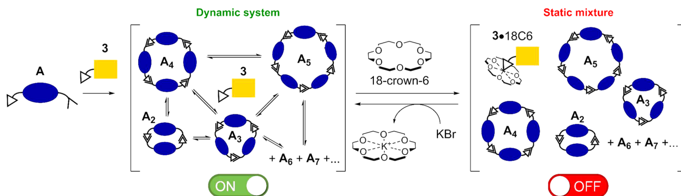
Figure 6. A dynamic mixture of macrocyclic oligomers of A is formed by aid of equilibrators 3 . The dynamic exchange of this mixture is then turned off by addition of 18-crown-6, which binds the equilibrators to form nonnucleophilic complex 3·18C6 . Turning the dynamic state of the system back on can be achieved by addition of a potassium salt, since the K^+ ion will competitively bind to 18-crown-6 and thereby liberate the equilibrators.
