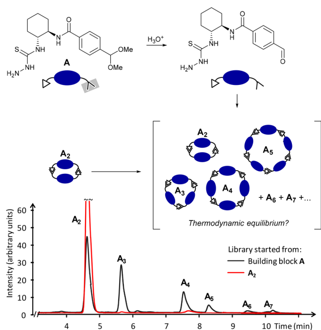
Figure 2. (Top) Schematic representation of acid-catalyzed hydrolysis of the acetal protecting group and subsequent macrocyclization. (Bottom) HPLC-UV chromatograms (at 325 nm) of libraries started from either building block A or from isolated macrocycle A 2 after 28 days of equilibration in CHCl 3 with 5 vol % TFA.
