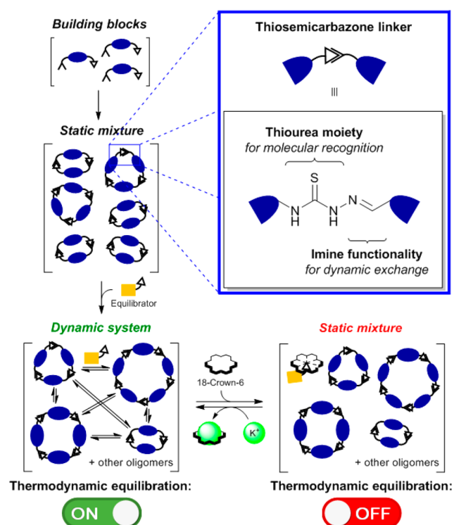
Figure 1. Principle of thiosemicarbazone-based dynamic systems presented in this study. Use of a nucleophilic catalyst, or equilibrator, allows for turning on or off the dynamic state of the system. (Inset) Structure of thiosemicarbazone motif, with thiourea and imine moieties highlighted.
