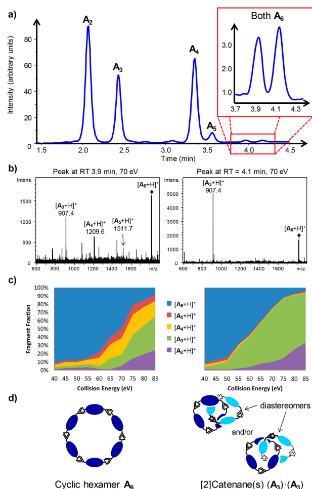
Figure 5. (a) HPLC-UV chromatogram (325 nm) of a library of building block A with peaks assigned on the basis of MS. (b) MS/MS at a collision cell energy of 70 eV of hexameric species at RT = 3.9 min (left) and RT = 4.1 min (right). (c) Distribution of intensities of hexameric, pentameric, tetrameric, trimeric, and dimeric ions in MS/MS analysis of both hexameric species as a function of applied collision cell energy. (d) Structural representations of distinct hexameric species corresponding to the peak at RT = 3.9 min (left) and 4.1 min (right).
