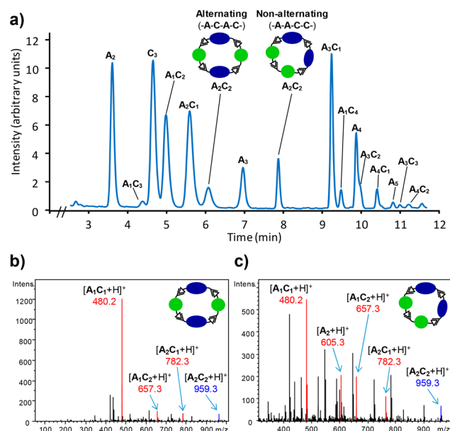
Figure 4. (a) HPLC-UV chromatogram (325 nm) of a library of building blocks A and C. (b) Tandem mass spectrometry (MS/MS) of the molecular ion ( m/z 959.3, shown in blue) of the A_2C_2 species eluting at ca. 6.1 min. (c) MS/MS of the molecular ion ( m/z 959.3, shown in blue) of the A_2C_2 species eluting at ca. 7.9 min. Fragment ions corresponding to loss of one or two monomer units are shown in red.
